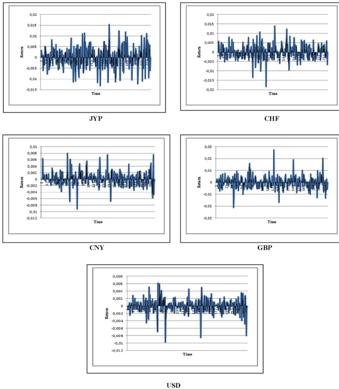
Fig. 1. Five Foreign Currency Return Chart
