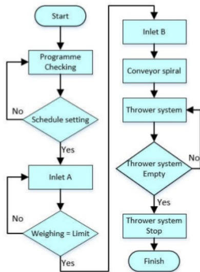
Figure 1. Workflow process of automatic feeder machine.
