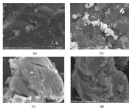
Figure 2. SEM images of \text{TiO}_2 /manganese composite with (a) 20wt%Mn, (b) 40wt%Mn, (c) 60wt%Mn, and (d) 80 wt%Mn and sintered at 1200^\circ\text{C} .
