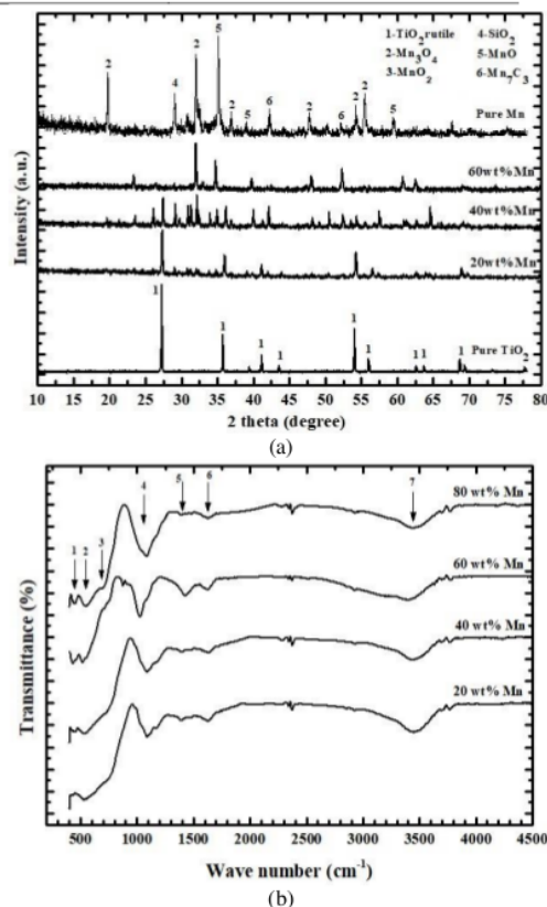
Figure 1. (a) XRD patterns and (b) FTIR spectra for TiO 2 /manganese composite with varying manganese content and sintered at 1200°C.
