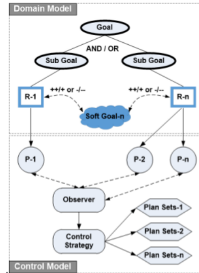
Figure 1. Conceptual model.
