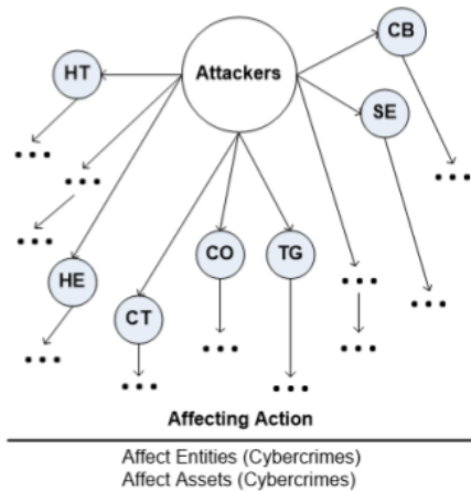
Figure 5. Attacker growth.
