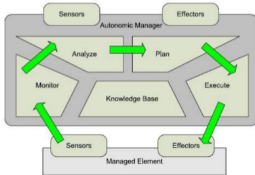
Figure 1. Process MAPE-K [7] [8].
