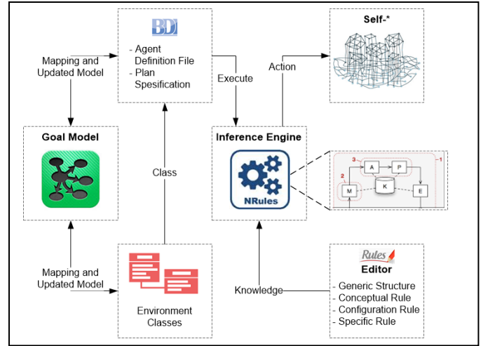
Figure 1. Self-adaptive framework.
