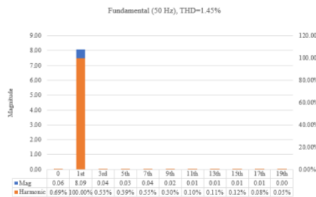
Fig. 9. Harmonic spectrum on inductive load testing after filter installation
