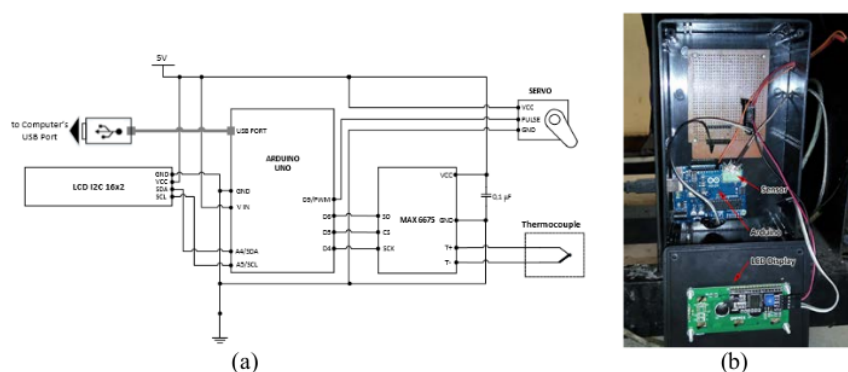
Figure 2. (a) Temperature control system circuit of the coconut sugar cooking system and (b) photograph of control system circuit.
