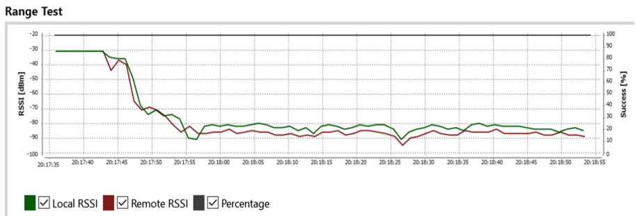
Fig. 9. The range result of the 1st test by using XCTU application at a depth of 0–5 m.
