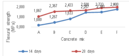
Fig. 5. Flexural Strength Graph of 14 and 28 Days Mixed Damdex Concrete and Bamboo Fiber
