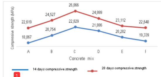
Fig. 1. Compressive Strength of Damdex Mixed Concrete and Bamboo Fiber 14 and 28 Days
