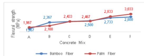
Fig. 8. The Flexural Strength of 28 Days Concrete a mixture of Damdex and Bamboo Fiber with a mixture of Damdex and Palm Fiber
