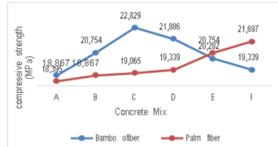
Fig. 3. Graph of 14 Days Concrete Compressive Strength between Mixed with Damdex and Bamboo Fiber with Mixed with Damdex and Palm Fiber
