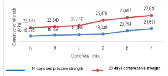
Fig. 2. Mixed Concrete Compressive Strength of Damdex and palm fiber 14 and 28 Days
