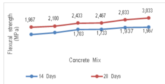
Fig. 6. Flexural Strength Graph of Damdex Mixed Concrete and 14 and 28 Day Fiber Ijuk
