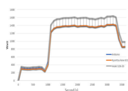
Figure 14. Active power measurement capture in comparison.
