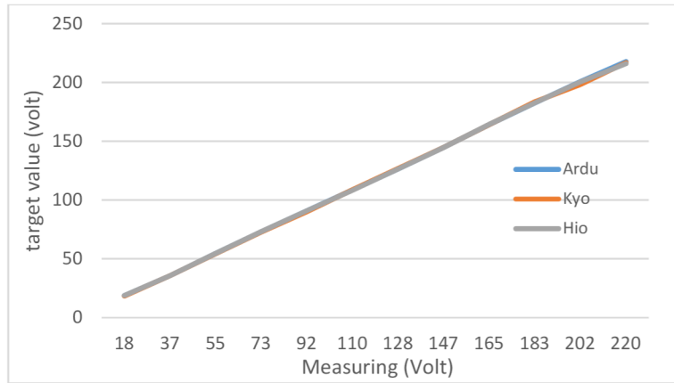
Figure 8. Testing of the accuracy of voltage measurement
