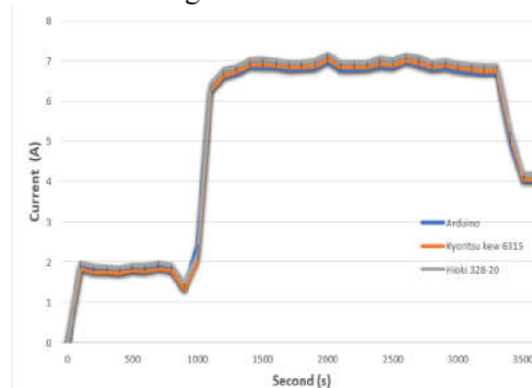
Figure 12. Current measurement capture in comparison.
