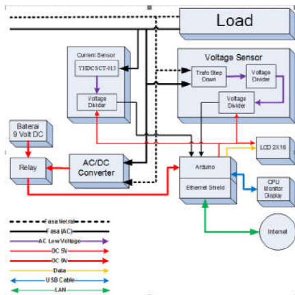
Figure 2. System architecture proposed.
