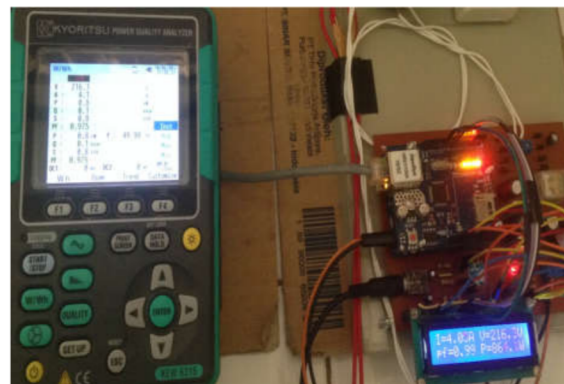
Figure 9(b). The comparison of measurement results.
