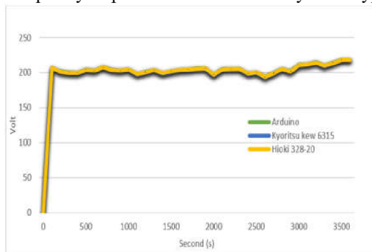
Figure 11. Voltage measurement value in comparison.
