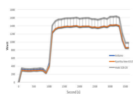
Figure 14. Active power measurement capture in comparison.
