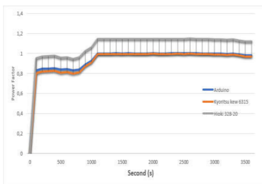
Figure 13. The power factor value measurements in comparison.
