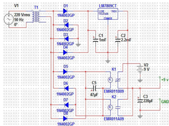
Figure 3. Circuit Scheme of backup power proposed.
