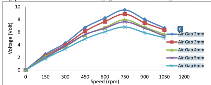
Figure 9. Relationship between output voltage and speed (rpm).
