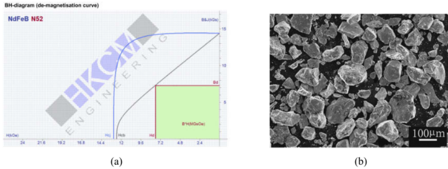
Figure 1. (a) Characteristic of NdFeB N52 [9], (b) SEM images of the magnetic powder of NdFeB. [8].
